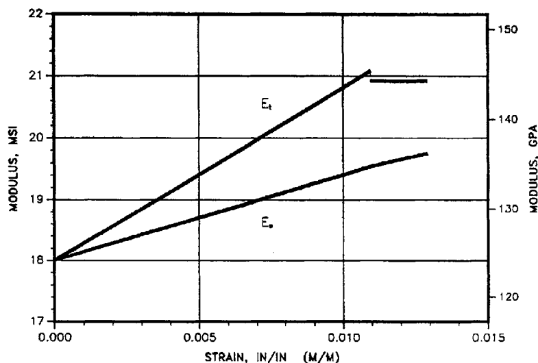
FIGURE 1.4.3(a) Modulus curves for AS4/3501-6, see Figure 8.4.4(a) (Volume 1).
