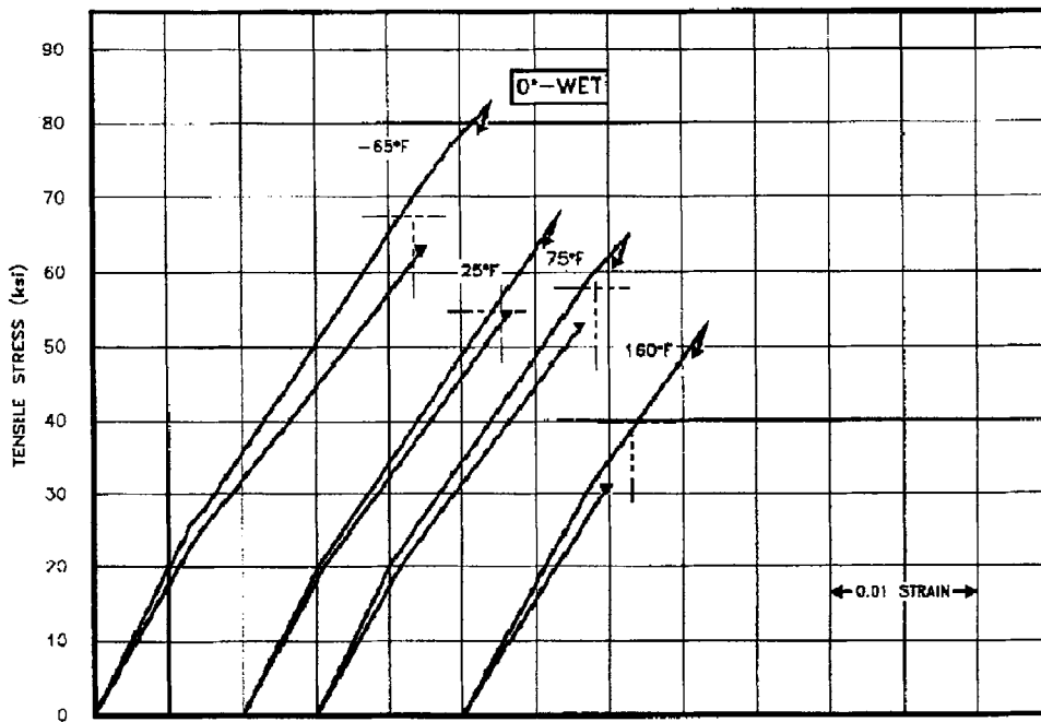
FIGURE A1.5.1(a) Tensile stress-strain for F-161/7781 fiberglass epoxy loaded in the 0° direction (31% resin).
