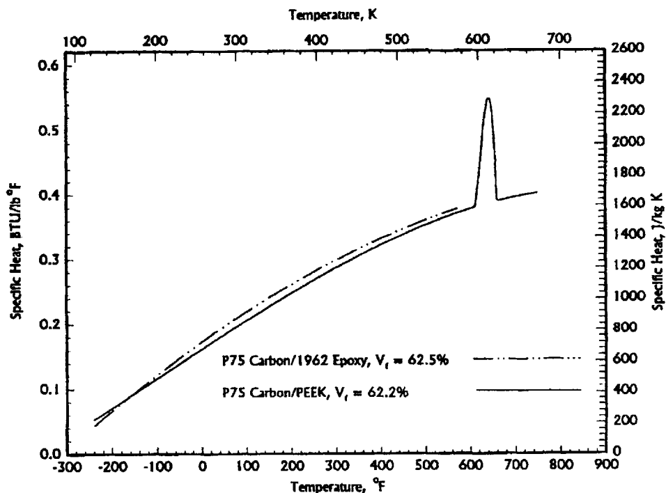
FIGURE 1.4.3(b) Specific heat of representative carbon fiber/polymer laminates as a function of temperature.
