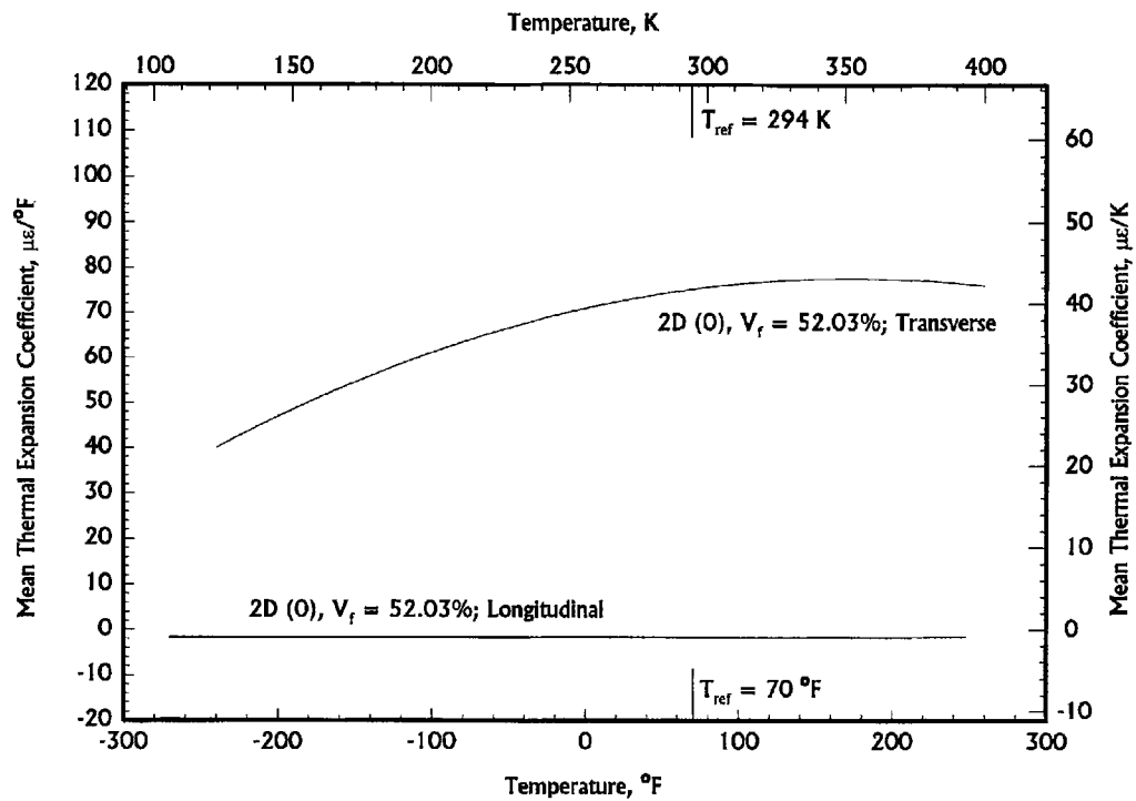
FIGURE 1.4.3(d) Mean coefficient of thermal expansion of representative carbon fiber/epoxy laminate (P75 carbon/1962 epoxy) as a function of temperature.
