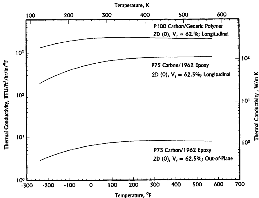
FIGURE 1.4.3(c) Thermal conductivity of representative carbon fiber/polymer laminates as a function of temperature.
